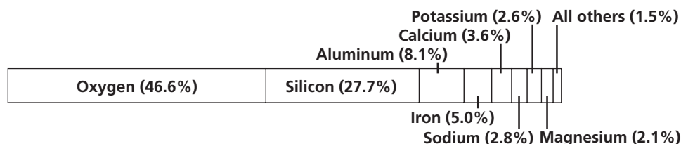
Elements in Earth's Crust
