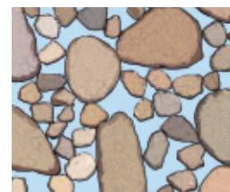
Poorly Sorted
